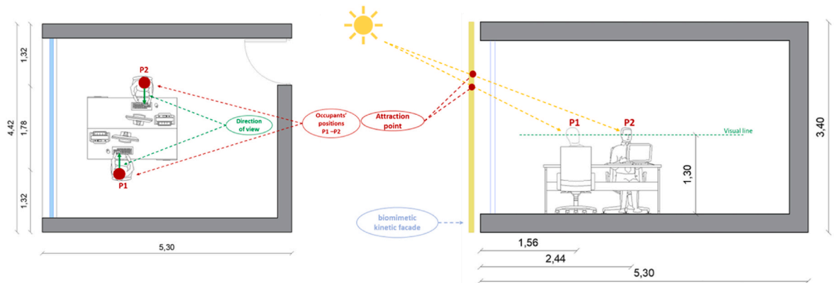
Fig. 8. Test room as an office building with occupant positions, direction of view, and attraction point. Left: floor plan; right: section.
