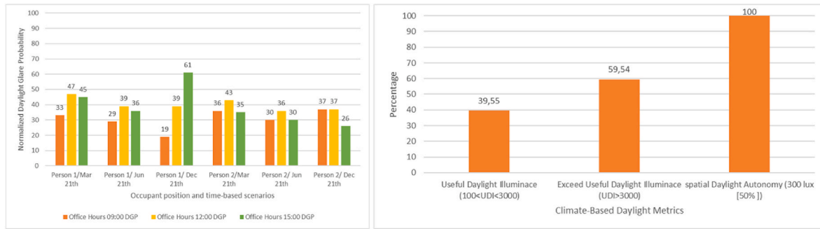
Fig. 10. Results of the parametric simulations related to the base case. Left: DGP values calculated on 21 March, 21 June and 21 December, at different office hours (9.00-12.00-15.00), occupant position and time-based scenarios. Right: Percentage mean of UDI, EUDI and sDA values.
