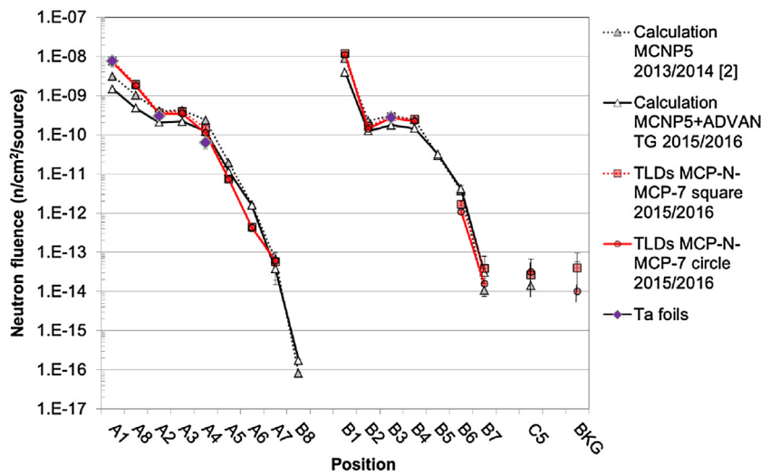
Fig. 5. Calculated and measured neutron fluence with TLDs and Ta foils. Calculations with MCNP5 using weight windows created by ADVANTG and previous calculation from Ref. [2] are both shown.
