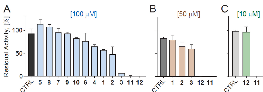
Fig. 3. (A, B, C) Residual activity (%) of hGAPDH upon incubation with (A) 100 \mu\text{M} of compounds 1–12 for 3 h; (B) 50 \mu\text{M} of compounds 1–3, 11, 12 for 30 min; (C) 10 \mu\text{M} of compounds 11 and 12 for 30 min. All experiments were performed at 25 ^{\circ}\text{C} in a buffered solution containing 10 mM TEA, 5 mM EDTA, 10 mM \text{KH}_2\text{PO}_4 , pH 7.6. hGAPDH was at 2 \mu\text{M} concentration. CTRL: activity of hGAPDH maintained under the same conditions in the absence of inhibitors. Experiments were performed in independent duplicates. Data are shown as mean \pm SD.
