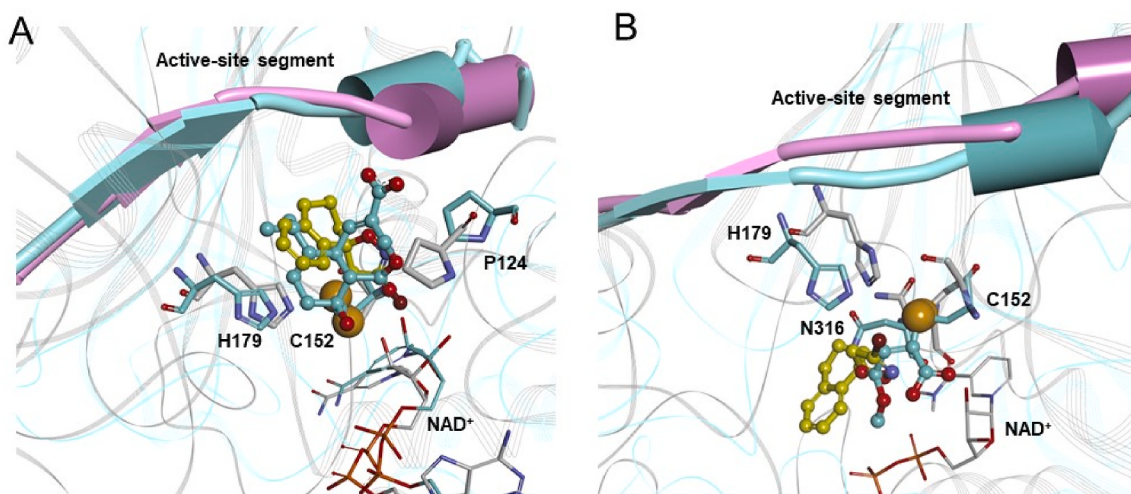
Fig. 7. Structural superimposition ( C\alpha atoms) of: (A) the ( S )-11/hGAPDH docked complex (ligand: ball&stick with carbon atoms colored in yellow; protein: line ribbon colored in grey and carbon atoms colored in white) on the X-ray structure of hGAPDH in complex with KA (KA: ball&stick with carbon atoms colored in cyan; protein: line ribbon and carbon atoms colored in cyan; PDB ID: 6M61); (B) the ( R )-11/hGAPDH docked complex (ligand: ball&stick with carbon atoms colored in yellow; protein: line ribbons colored in grey and carbon atoms colored in white) on the X-ray structure of hGAPDH in complex with MMF (MMF: ball&stick with carbon atoms colored in cyan; protein: line ribbon and carbon atoms colored in cyan; PDB ID: 6IQ6). The interacting residues and NAD^+ (carbon atoms colored in white) are displayed in stick. The sulfur atom of C152 is displayed in CPK (scaled by 50%). Ligands, KA, MMF, NAD^+ , and residues are colored by atom type (N = blue, O = red, S = yellow, P = orange, Br = brown). Hydrogen atoms are omitted for clarity.
