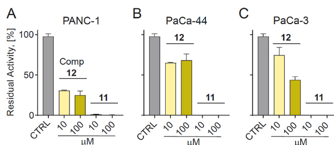
Fig. 11. Percent activity (%) of hGAPDH in cell lysates of PANC-1 (a), PaCa-44 (b), and PaCa-3 (c) upon incubation with either compounds 11 or 12 at 0 (CTRL), 10 or 100 \mu M concentration. The activity was normalized to the total protein content. Experiments were performed in independent duplicates. Data are shown as mean \pm SD.
