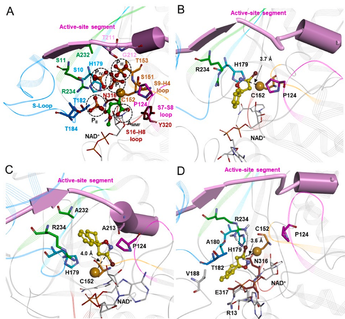
Fig. 6. (A) hGAPDH (PDB ID: 1ZNQ) active site substructures involved in the interaction with substrate, inhibitors, and anions. The key interaction residues are displayed and labelled. The binding sites P_I - P_{IV} and A_{MMF} are highlighted with black dashed circles. (B) Docked complex of (S)-1/hGAPDH. (C) Docked complex of (S)-11/hGAPDH. (D) Docked complex of (R)-11/hGAPDH. The structure of hGAPDH is displayed as line ribbon and colored in grey. The S7-S8 loop (aa122-129) is colored in magenta, the S9-H14 loop (aa149-153) in orange, the S10 strand (aa171-180) in cyan, the S-loop (aa181-207) in light blue, the S11 strand (aa228-235) in green, and the S16-H8 loop (aa315-320) in brown. The active-site segment (aa208-220) is displayed in cartoon form and colored in pink. Phosphate ions, mono-methyl fumarate (MMF, carbon atoms colored in green) and ligands (carbon atoms colored in yellow) are displayed in ball&stick while the interacting residues and NAD^+ (carbon atoms colored in white) in stick. The sulfur atom of C152 is displayed in CPK (scaled by 50%). The distance between the electrophilic carbon C3 of BDHI ring and the C152 sulfur atom is showed (B-D). Hydrogen atoms are omitted for clarity, except those involved in hydrogen bond interactions (black dashed lines).
