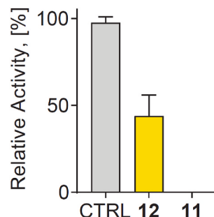
Fig. 10. Relative activity (%) of hGAPDH upon incubation with 10 \mu M of compounds 11 and 12 for 48 h at 37 °C in a buffered solution containing 10 mM TEA, 5 mM EDTA, 10 mM KH 2 PO 4 , pH 7.6. hGAPDH concentration: 2 \mu M. CTRL: non-treated hGAPDH activity. Experiments were performed in independent duplicates. Data are shown as mean \pm SD.
