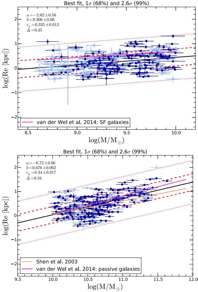
Fig. 18. Best-fit of the mass-size relation in Eq. (6) for early-type passive low-mass galaxies ( M_\star \leq 10^{10} M_\odot ; upper panel) and high-mass galaxies ( M_\star > 10^{10} M_\odot ). The best-fit values of the two parameters a and b with their 1\sigma uncertainty are given in the two panels. Dark blue points identify spectroscopic members, while light blue point are photometric members.
