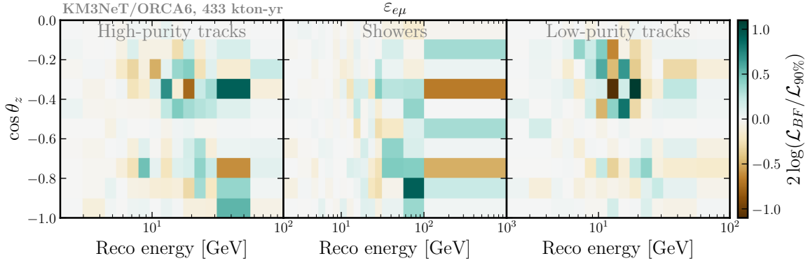
Figure 13. Bin-by-bin contribution to the log-likelihood ratio of the best-fit hypothesis over the point |\varepsilon_{e\mu}| = 0.055 . From left to right, the three panels show the contributions arising from the high-purity tracks, showers and low-purity tracks.
