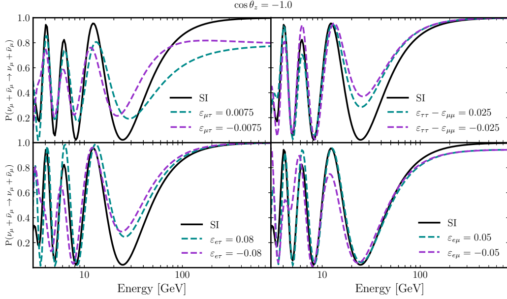
Figure 1. Combined \nu_\mu + \bar{\nu}_\mu survival probability for neutrinos propagating along the up-going, Earth core-crossing trajectory \cos\theta_z = -1 . The standard interaction prediction (SI) is represented by the solid black line, and is identical for the four subplots. Dashed lines show the NSI expectation for positive and negative coupling strength in the cases of non-zero \varepsilon_{\mu\tau} (top left), \varepsilon_{\tau\tau} - \varepsilon_{\mu\mu} (top right), \varepsilon_{e\tau} (bottom left) and \varepsilon_{e\mu} (bottom right). The specific values of NSI parameters were chosen for visualisation purposes. For all curves, the standard oscillation parameters \Delta m_{ij}^2 and \theta_{ij} were fixed at NuFit 5.0 [6] for normal ordering (NO).
