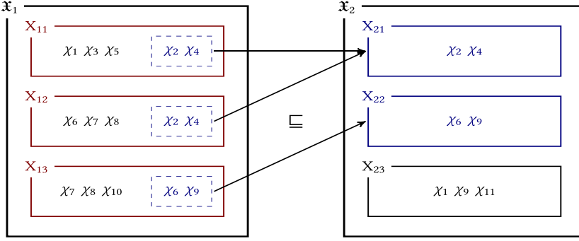
Fig. 1. The preorder \sqsubseteq on hyperassignments: for every X_{1i} \in \mathfrak{X}_1 , there is a X_{2j} \in \mathfrak{X}_2 with X_{2j} \subseteq X_{1i} . More than one set in \mathfrak{X}_1 may be related to the same set in \mathfrak{X}_2 ; there may be sets in \mathfrak{X}_2 not related to any set in \mathfrak{X}_1 .
