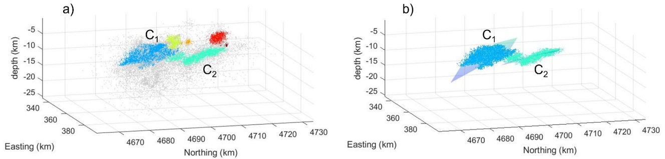
Figure 2. A workflow application to L'Aquila seismic sequence. (a) A DBSCAN solution illuminating six earthquake clusters ( Z = 200 and \epsilon = 0.5 km). Gray points are earthquakes discarded as noise points. (b) First-order planar surfaces retrieved by principal component analysis are shown for the two biggest clusters C_1 and C_2 .
