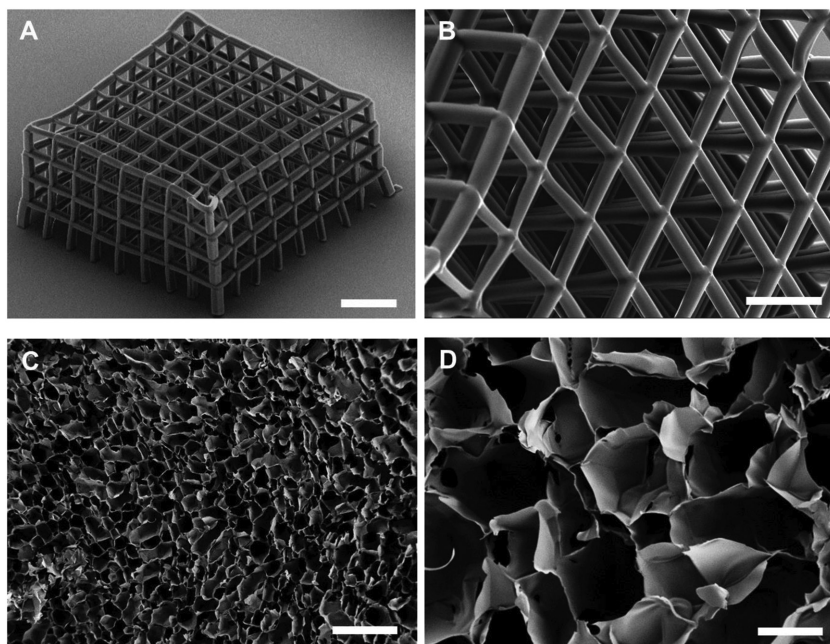
Figure 1. SEM characterization of fabricated scaffolds. A,B) Ormocomp ordered scaffolds fabricated by means of 2-photon patterning. C,D) PEDOT:PSS scaffolds prepared by the ice-templating technique. Scale bars: A) 150 \mu\text{m} , B) 50 \mu\text{m} , C) 400 \mu\text{m} , D) 100 \mu\text{m} , inset D) 200 \mu\text{m} .
