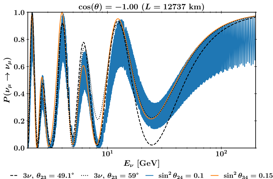
Figure 5. Muon neutrino survival probability as a function of the neutrino energy under various scenarios for \cos \theta = -1.0 . The three-flavour standard oscillation model assuming the nominal value for \theta_{23} = 49.1^\circ (dashed black) is compared with the three-flavour model with \theta_{23} = 59^\circ (dotted black) and with the 3+1 models with \sin^2 \theta_{24} = 0.1 (blue) and \sin^2 \theta_{34} = 0.15 (orange), for \Delta m_{41}^2 = 1 \text{ eV}^2 . All other sterile parameters are set to 0.
