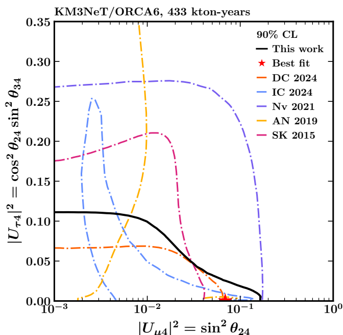
Figure 6. Comparison of the upper limits at 90% CL on |U_{\mu 4}|^2 and |U_{\tau 4}|^2 obtained by ORCA6 with previous measurements from Super-Kamiokande (SK) [16], NOvA (Nv) [66], ANTARES (AN) [17], IceCube (IC) [10] and DeepCore (DC) [11]. The excluded regions are on the top right side of the contours.
