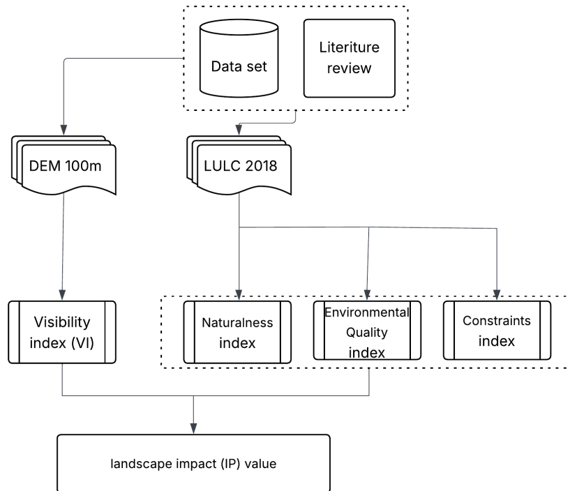
Fig.1 Methodology framework
