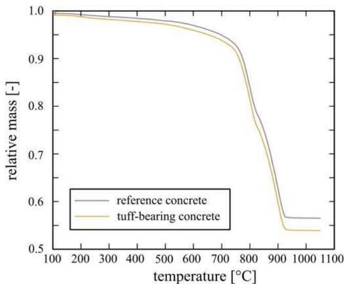
Fig. 2. Relative mass of the reference concrete (grey curve) and the tuff-bearing concrete (yellow curve) as a function of temperature (up to 1050 °C). Sample (powders) masses were 69.2 and 74.4 mg for the reference and tuff-bearing concrete, respectively. Samples were heated at a rate of 25 °C/min (see methods section for details). (For interpretation of the references to colour in this figure legend, the reader is referred to the Web version of this article.)
