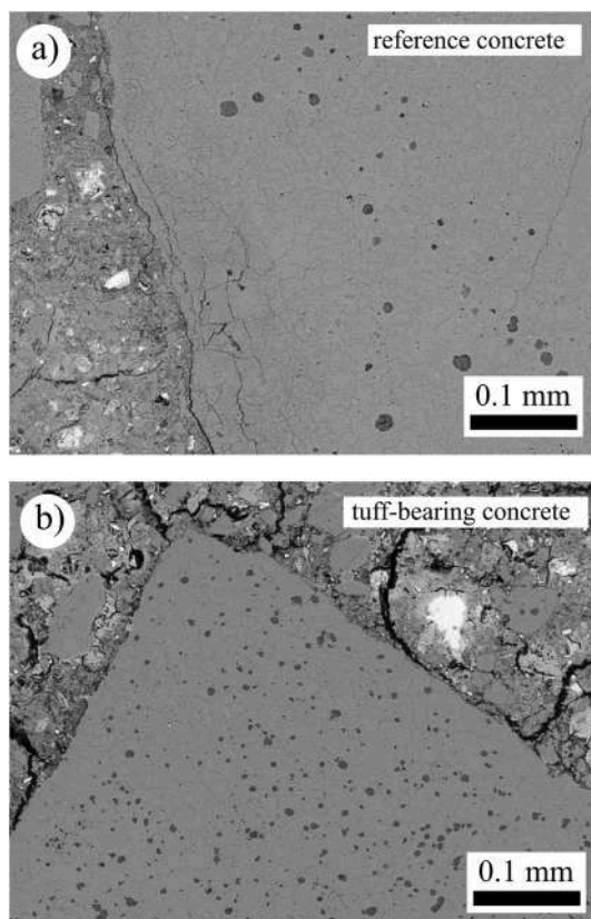
Fig. 8. Backscattered scanning electron microscope images showing microcracks and sub-circular pores within the aggregates of (a) the reference concrete and (b) the tuff-bearing concrete following exposure to 750 °C.
