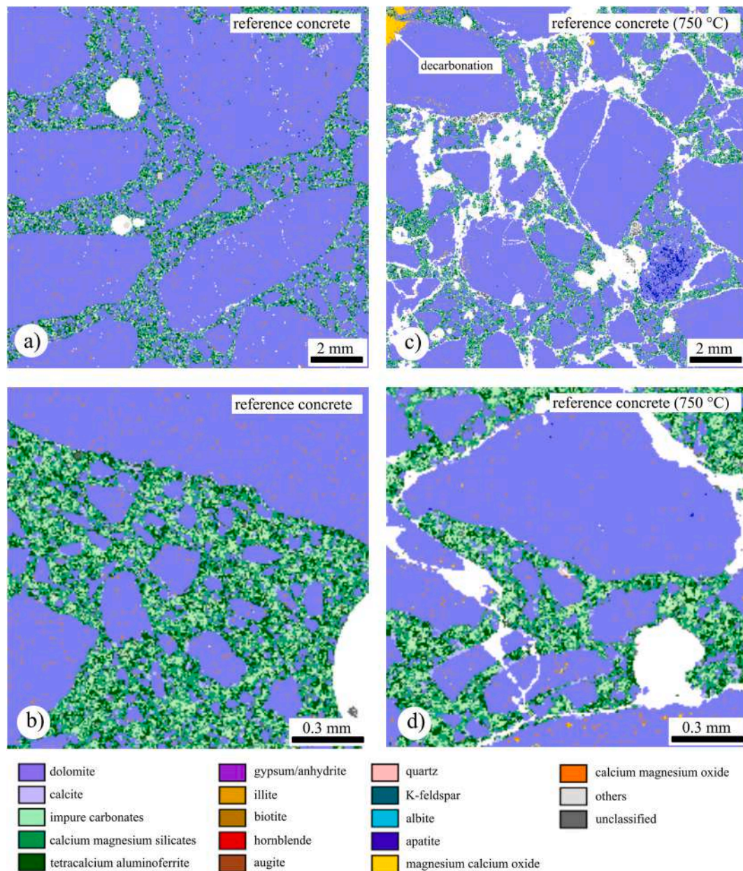
Fig. 9. QEMSCAN™ (Quantitative Evaluation of Minerals by Scanning Electron Microscopy) mineral composition maps for the as-prepared reference concrete at (a) a step size of 20 \mu\text{m} and (b) a step size of 2 \mu\text{m} , and the reference concrete following exposure to 750 ^{\circ}\text{C} at (c) a step size of 20 \mu\text{m} , and (d) a step size of 2 \mu\text{m} .
