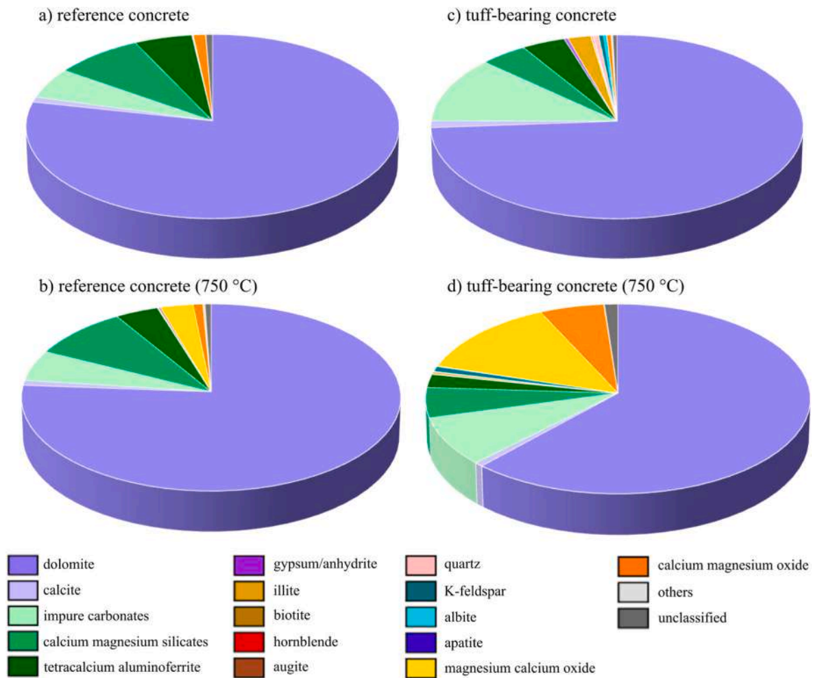
Fig. 11. Pie charts showing the mineral composition (as quantified by the QEMSCAN™) of (a) the as-prepared reference concrete, (b) the reference concrete following exposure to 750 °C, (c) the as-prepared tuff-bearing concrete, and (d) the tuff-bearing concrete following exposure to 750 °C (the data are also available in Table 4).
