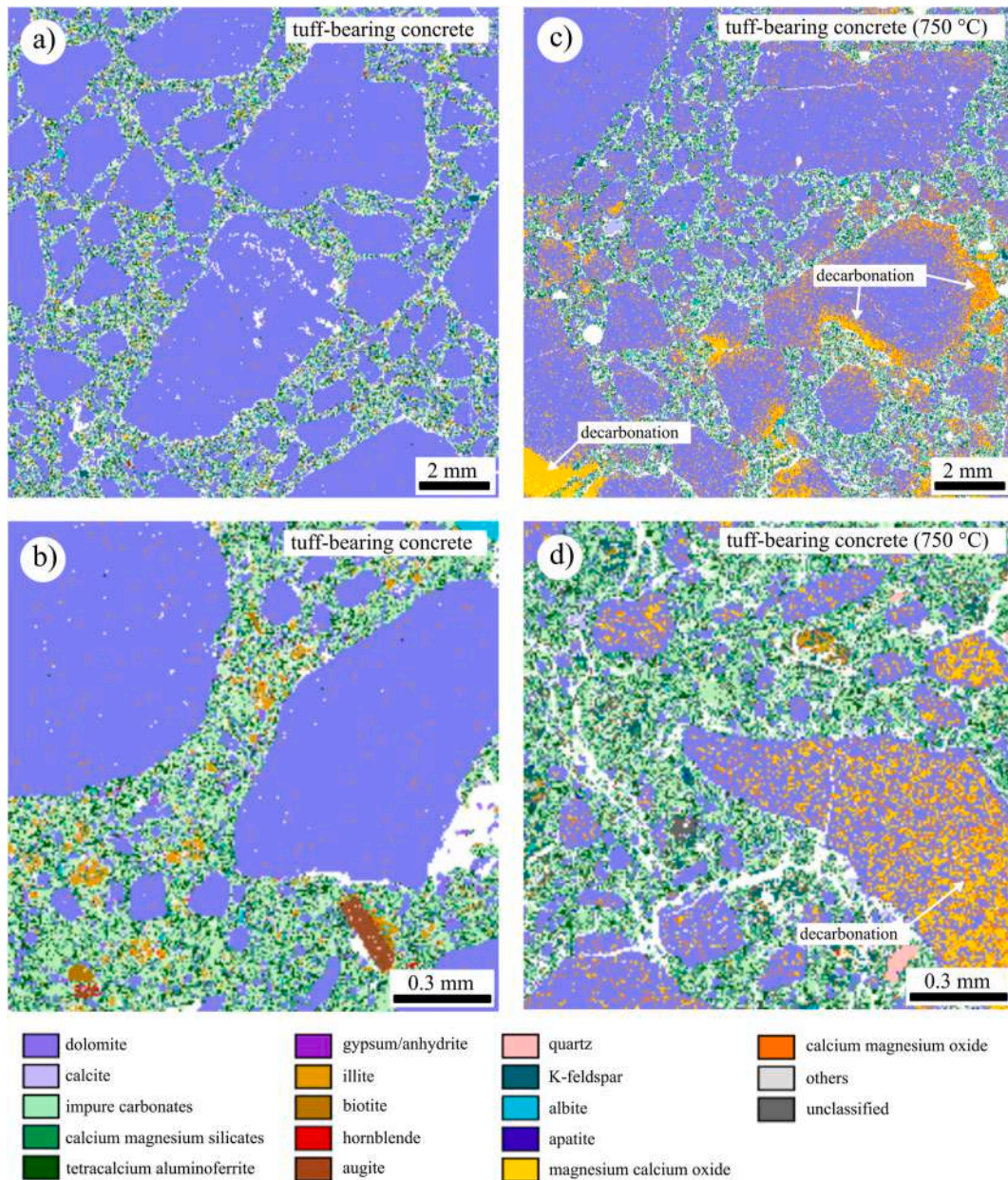
Fig. 10. QEMSCAN™ (Quantitative Evaluation of Minerals by Scanning Electron Microscopy) mineral composition maps for the as-prepared tuff-bearing concrete at (a) a step size of 20 μm and (b) a step size of 2 μm, and the tuff-bearing concrete following exposure to 750 °C at (c) a step size of 20 μm, and (d) a step size of 2 μm.
