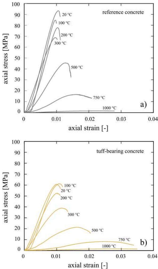
Fig. 5. Representative uniaxial stress-strain curves for as-prepared and thermally stressed samples of (a) the reference concrete and (b) the tuff-bearing concrete. The temperature next to each curve indicates the thermal stressing temperature.
