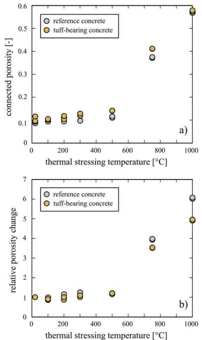
Fig. 4. (a) Connected porosity as a function of thermal stressing temperature for the reference concrete (grey circles) and the tuff-bearing concrete (yellow circles). (b) Relative porosity change (as a fraction) as a function of thermal stressing temperature for the reference concrete (grey circles) and the tuff-bearing concrete (yellow circles). (For interpretation of the references to colour in this figure legend, the reader is referred to the Web version of this article.)
