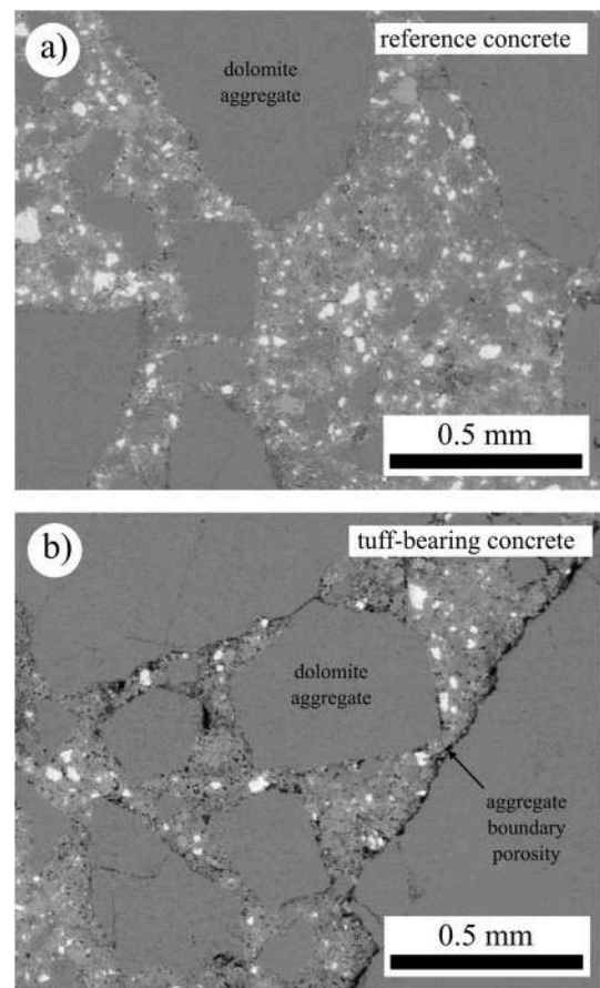
Fig. 1. Backscattered scanning electron microscope images of (a) the as-prepared reference concrete and (b) the tuff-bearing concrete (b). See Table 1 for mix ingredients and proportions.
