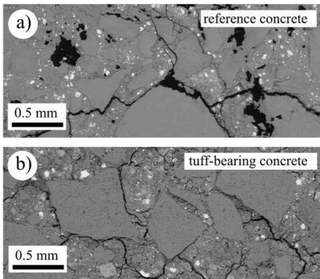
Fig. 7. Backscattered scanning electron microscope images showing microcracks within the (a) reference concrete and (b) the tuff-bearing concrete following exposure to 750 °C.
