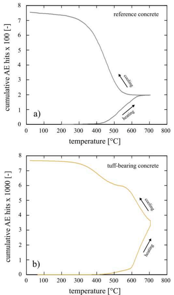
Fig. 3. The number of detected acoustic emission hits during the heating and cooling (at 1 °C/min) of (a) the reference concrete and (b) the tuff-bearing concrete.
