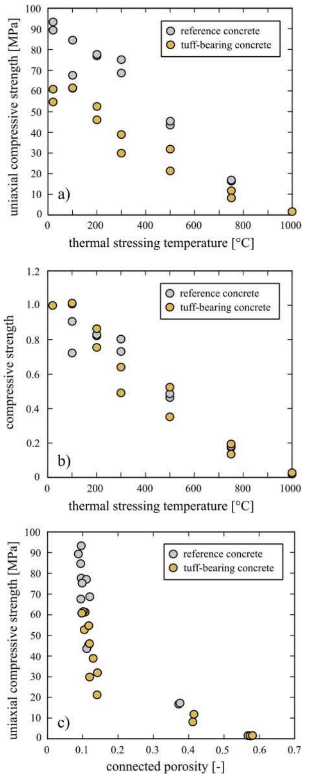
Fig. 6. (a) Residual uniaxial compressive strength as a function of thermal stressing temperature for the reference concrete (grey circles) and the tuff-bearing concrete (yellow circles). (b) Relative residual uniaxial compressive strength (as a fraction) as a function of thermal stressing temperature for the reference concrete (grey circles) and the tuff-bearing concrete (yellow circles). (c) Residual uniaxial compressive strength as a function of connected porosity for the reference concrete (grey circles) and the tuff-bearing concrete (yellow circles). (For interpretation of the references to colour in this figure legend, the reader is referred to the Web version of this article.)
