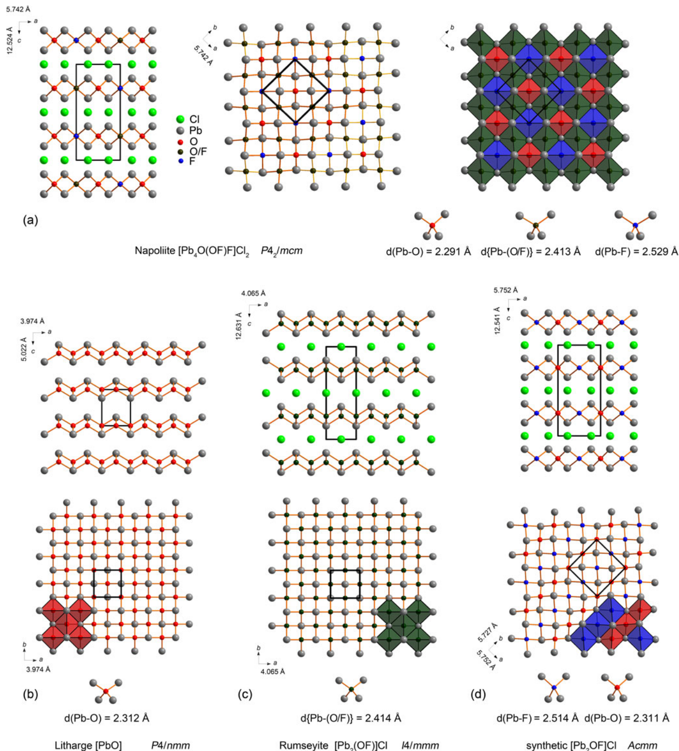
Figure 4. The crystal structures in balls-and-sticks and polyhedral representations of (a) napoliite; (b) structurally related litharge (Boher et al. , 1985); (c) rumseyite (Turner et al. , 2012); and (d) synthetic [\text{Pb}_2\text{OF}]\text{Cl} (Aurivillius, 1977). In structural formulae, litharge-derived blocks are given in square brackets. Average Pb–X (X = O, F) bond lengths in \text{XPb}_4 anion-centred tetrahedra are given for each crystal structure. Designations: grey balls = Pb; green balls = Cl; red balls = O sites; blue balls = F sites; dark green = mixed O/F sites; \text{OPb}_4 tetrahedra = red; (\text{O}/\text{F})\text{Pb}_4 tetrahedra = dark green and \text{FPb}_4 = blue. Pb–Cl long bonds are omitted for clarity.
