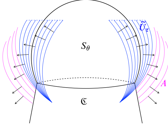
Figure 4. The foliations defined in Theorem 4.11.
