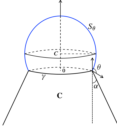
Figure 1. The spherical cap S_\theta lying on \mathbf{C} has radius r = \frac{1}{\sin \theta} and center at C = (0, 0, -\frac{1}{\tan \theta}) .
