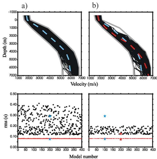
Figure 2. (a) Randomly generated initial 1-D velocity models. The upper and lower velocity bounds (solid gray lines) and the 1-D velocity model from Zollo et al. [2003] (dashed cyan line) are also shown. (bottom left) Initial (black points) and final misfit values (red points) obtained from inversions. Cyan stars indicate the initial and the final misfit values for the 1-D velocity model of Zollo et al. [2003]. (b) Same as Figure 2a, after the selection described in the text.
