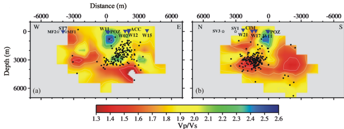
Figure 10. Vertical cross sections describing the variation of the V_p/V_s ratio and earthquake distribution (black points) along the (a) E-W and (b) N-S directions reported in Figure 1. Black stars and triangles indicate well and station locations.
