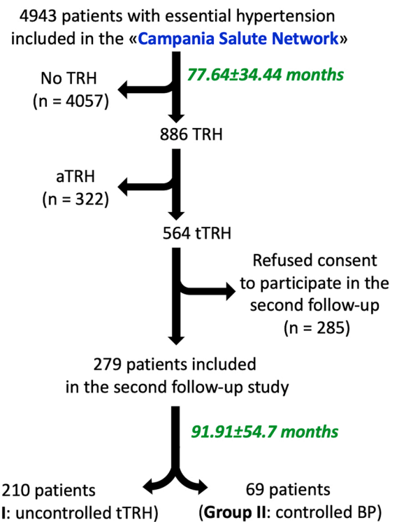
Fig. 1. Flowchart of the study. TRH: therapy-resistant hypertension; aTRH: apparent therapy-resistant hypertension; BP: blood pressure; tTRH: true therapy-resistant hypertension.
