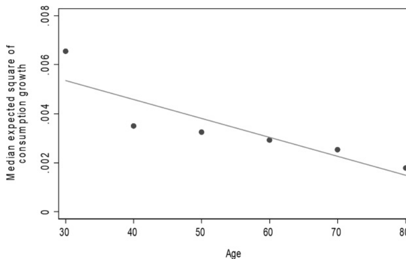
FIGURE 2.—EXPECTED SQUARE OF CONSUMPTION GROWTH, BY AGE GROUPS
