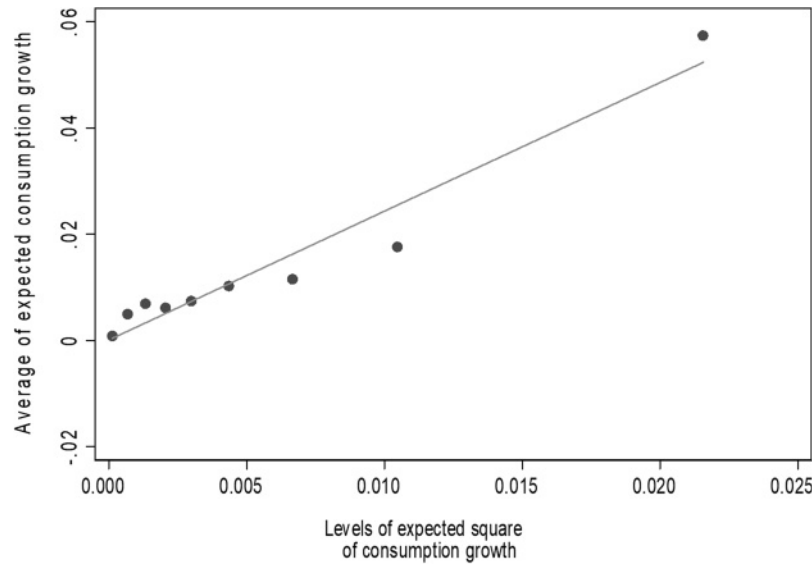
FIGURE 3.—EXPECTED CONSUMPTION GROWTH, BY GROUPED VALUES OF EXPECTED SQUARE OF CONSUMPTION GROWTH
