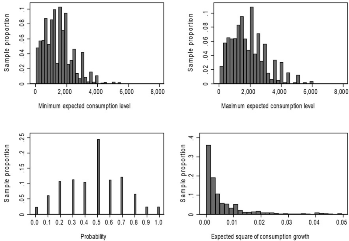
FIGURE 1.—THE DISTRIBUTION OF EXPECTED CONSUMPTION
