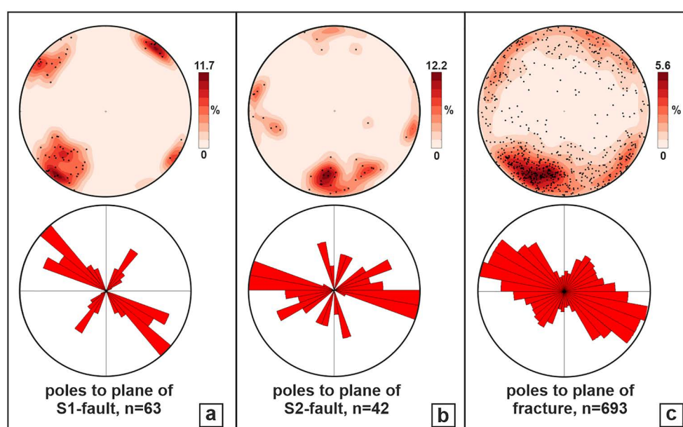
Figure 8. Stereographic projections (lower hemisphere, equiareal net) of the fault and fracture poles and corresponding rose diagrams.
