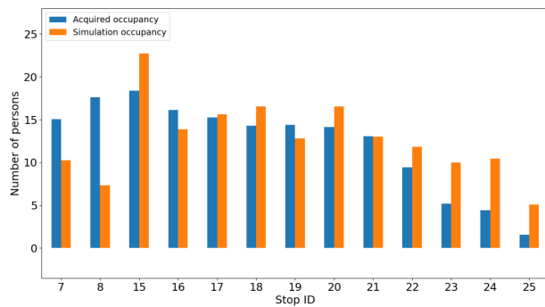
Figure 4: Average occupancy for Route 003
