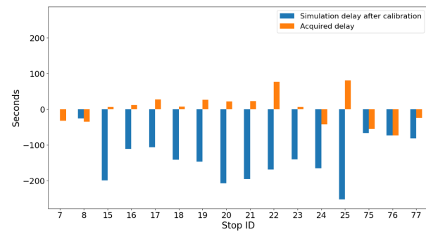
(b) Simulated delay and real one, for line 003
