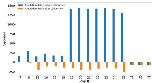
(a) Delay of line 003, before and after the calibration step
