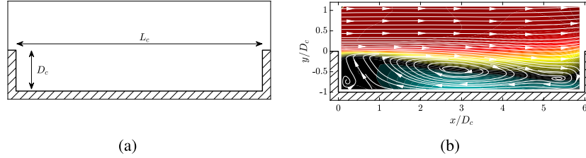
Fig. 3. Open cavity flows. Panel (a): geometrical sketch; panel (b): mean streamwise velocity component and streamlines distribution. Data courtesy of Zhang et al. [48]. (■ blue, cyan, black, yellow, red, -1 < \bar{u}/\|\bar{u}\|_{\infty} < 1 ).
