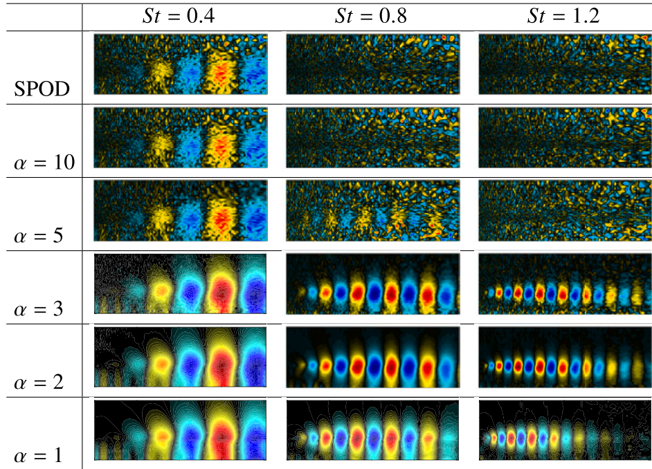
Fig. 7. Comparison between SPOD and robust SPOD leading modes at different St . Gaussian noise with the 10% of corrupted data points. Panels in the first line refer to SPOD modes of corrupted data. Other rows show the effect of the de-noising parameter \alpha on the robust SPOD modes. Data corruption is modeled as Gaussian noise with \pm 4p_{\max} variance. In all the panels, the abscissa and ordinate are the dimensionless axial coordinate x/D_j and radial coordinate r/D_j , respectively, omitted for clarity. Field variables have been normalized with respect to their maximum. ( 0 < x/D_j < 4 and 0 < r/D_j < 1.5 , blue, cyan, black, yellow, red, -1 < \phi_{f_k}/\|\phi_{f_k}\|_{\infty} < 1 ).
