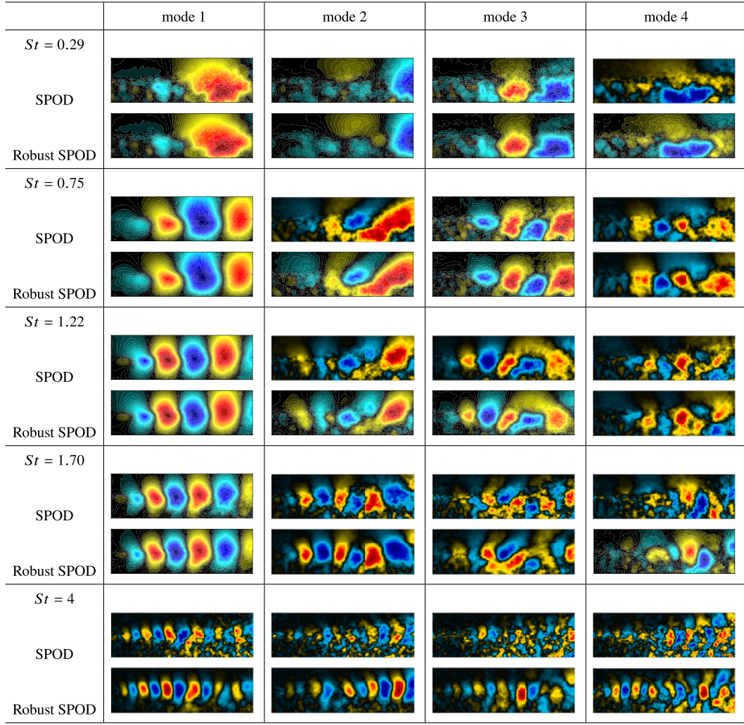
Fig. 16. Comparison between SPOD and robust SPOD leading v modes at different St . Field variables have been normalized with respect to their maximum. Note that for robust SPOD the Algorithm 3 has been employed. De-noising parameter \alpha = 1 . In all the panels, the abscissa and ordinate are the dimensionless axial coordinate x/D_c and radial coordinate r/D_c , respectively, omitted for clarity. (blue, cyan, black, yellow, red, -1 < \phi_{f_k} / \|\phi_{f_k}\|_\infty < 1 ).
