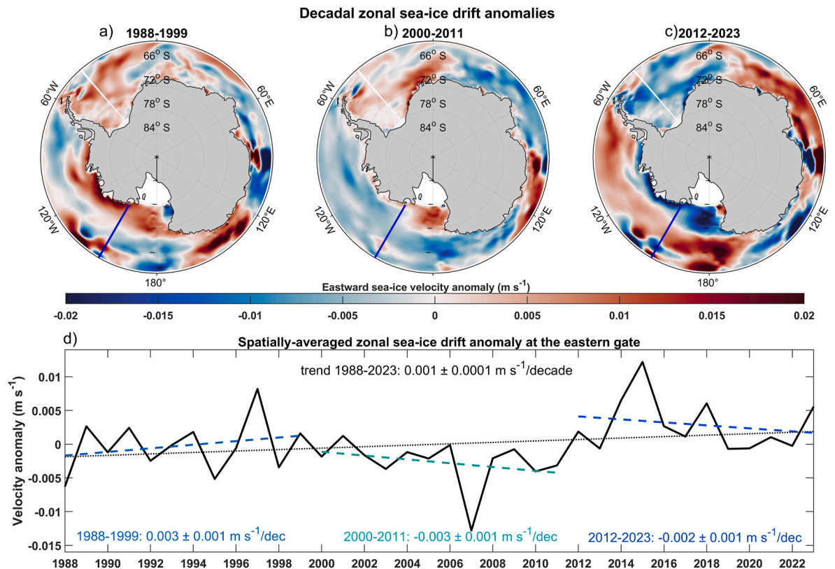
Fig. 5. Spatial distribution of the de-seasoned eastward sea ice drift anomalies during (a) 1988–1999, (b) 2000–2011 and (c) 2012–2023. The overall mean and seasonal climatological fields of the zonal sea ice drift can be seen in Fig. S2 in the supplementary material; (d) Yearly values of the spatially-averaged anomalies at the eastern gate with trends per individual ~ decadal period (colored dashed lines) and trend for the entire time span (black dotted line). The longitudinal section of the eastern gate is indicated with a thick blue line in the spatial maps (a)–(c).
