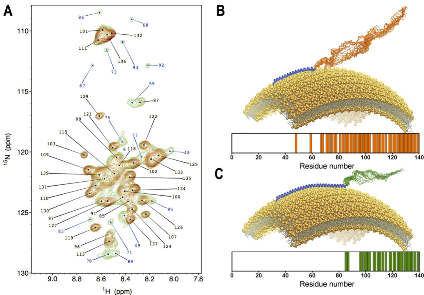
Figure 1. Disordered regions of \alpha\text{S} bound to mitochondrial-like membranes probed by ssNMR. (A) ^1\text{H} -detected ^1\text{H} - ^{15}\text{N} -HSQC ssNMR of \alpha\text{S} bound to OMM (green spectrum) and OMM CL+ (red spectrum). Spectra were measured at 25 °C using MAS ssNMR using a 3.2 mm E^{\text{Free}} probe with spinning rate of 12.5 kHz, and a ^1\text{H} Larmor frequency of 700 MHz. The assignment of the spectra was derived by superimposing the ^1\text{H} - ^{15}\text{N} -HSQC ssNMR with previously assigned spectra in solution NMR of unbound \alpha\text{S} . 54 Residues whose resonances are present only in the OMM-bound spectrum are labeled in blue. Residues whose resonances are present in both spectra are labeled in black. (B, C) Representation of SUV-bound \alpha\text{S} . Schematic illustration of the binding mode of \alpha\text{S} to OMM (B) and OMM CL+ (C) vesicles. Bar plots indicate the residues numbers of resonances found in the ^1\text{H} - ^{15}\text{N} -HSQC ssNMR of \alpha\text{S} -OMM (B) and \alpha\text{S} -OMM CL+ (C). (B) In the case of OMM, numerous residues maintained enough conformational disorder to be detected by ^1\text{H} - ^{15}\text{N} -HSQC ssNMR, including a number of residues in the central region. Orange and blue ribbons represent disordered and helical-structured regions of \alpha\text{S} bound to OMM. (C) In the case of OMM CL+ the number of residues that maintain disorder and poor association with the membrane is reduced significantly in the central region. Green and blue ribbons represent disordered and helical-structured regions of \alpha\text{S} bound to OMM CL+ .
