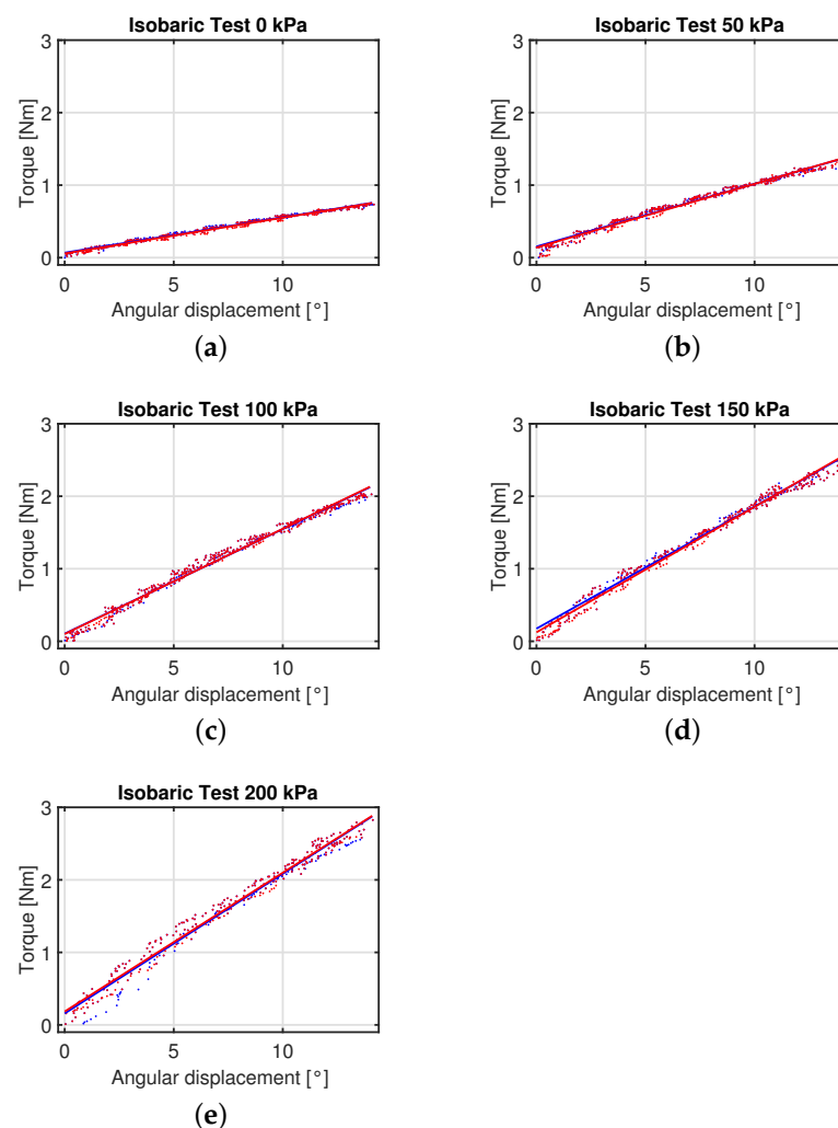
Figure 10. Isobaric tests. Expansion (in blue) and compression (in red) for the soft actuator at 0 kPa (a), 50 kPa (b), 100 kPa (c), 150 kPa (d), and 200 kPa (e).
