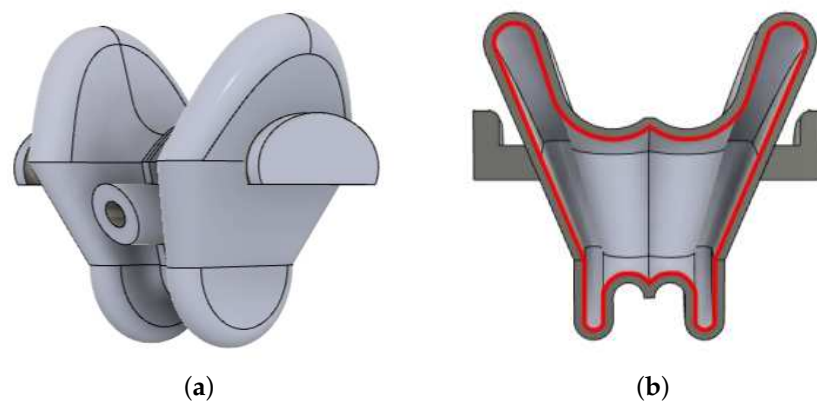
Figure 4. Pneumatic soft actuator (a) and air chamber with auxetic structure (b).
