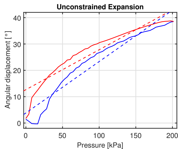
Figure 8. Unconstrained expansion: characterisation curves. Expansion (blue solid line) and compression (red solid line) curves; regression lines (dashed).
