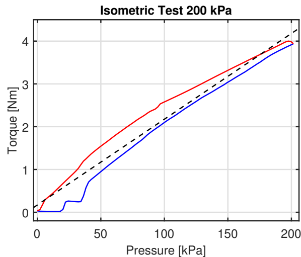
Figure 9. Isometric test at 200 kPa. Expansion (blue solid line) and compression (red solid line) curves; regression line (dashed).
