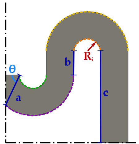
Figure 2. REH auxetic path with rounded corners.
