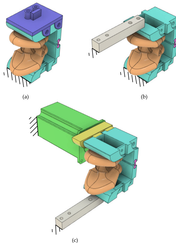
Figure 7. CAD representation for the different setups for unconstrained expansion (a), isometric (b), and isobaric (c) characterisation.
