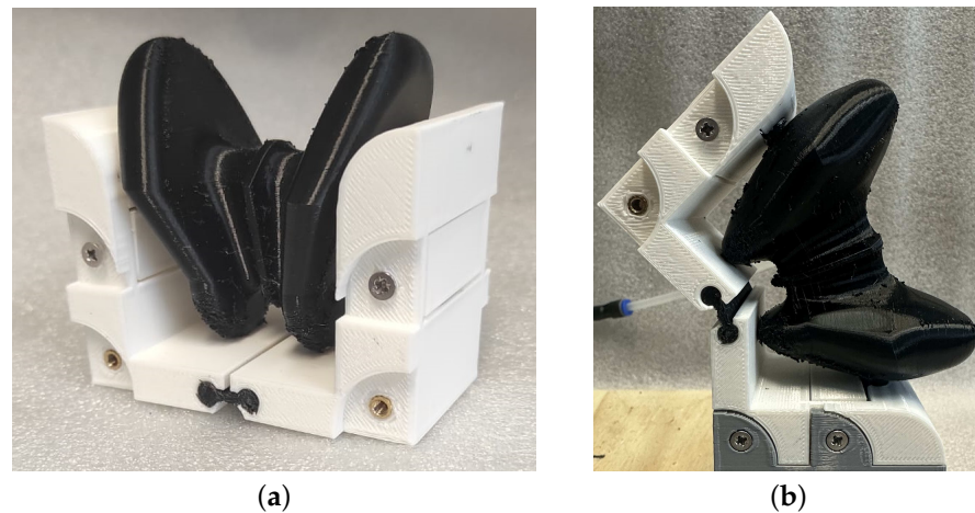
Figure 6. Photo of the real setup of the hybrid actuator: soft air chamber (in TPU, black) and rigid frames (in PLA, white) in nominal (a,b) inflated state.
