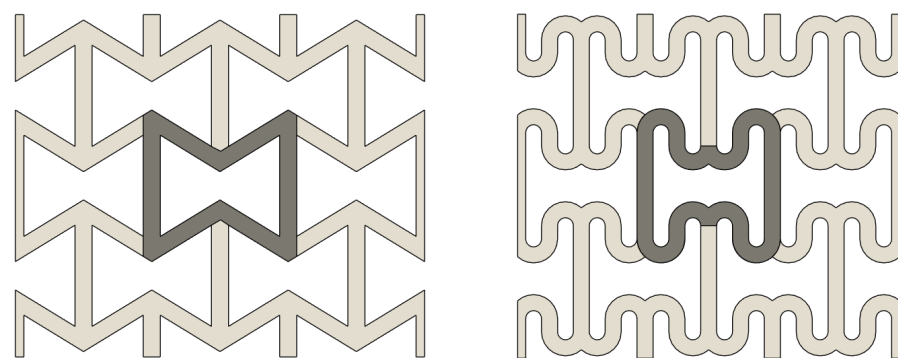
Figure 1. Re-entrant honeycomb (REH): classical (on the left) and with rounded corners (on the right).
