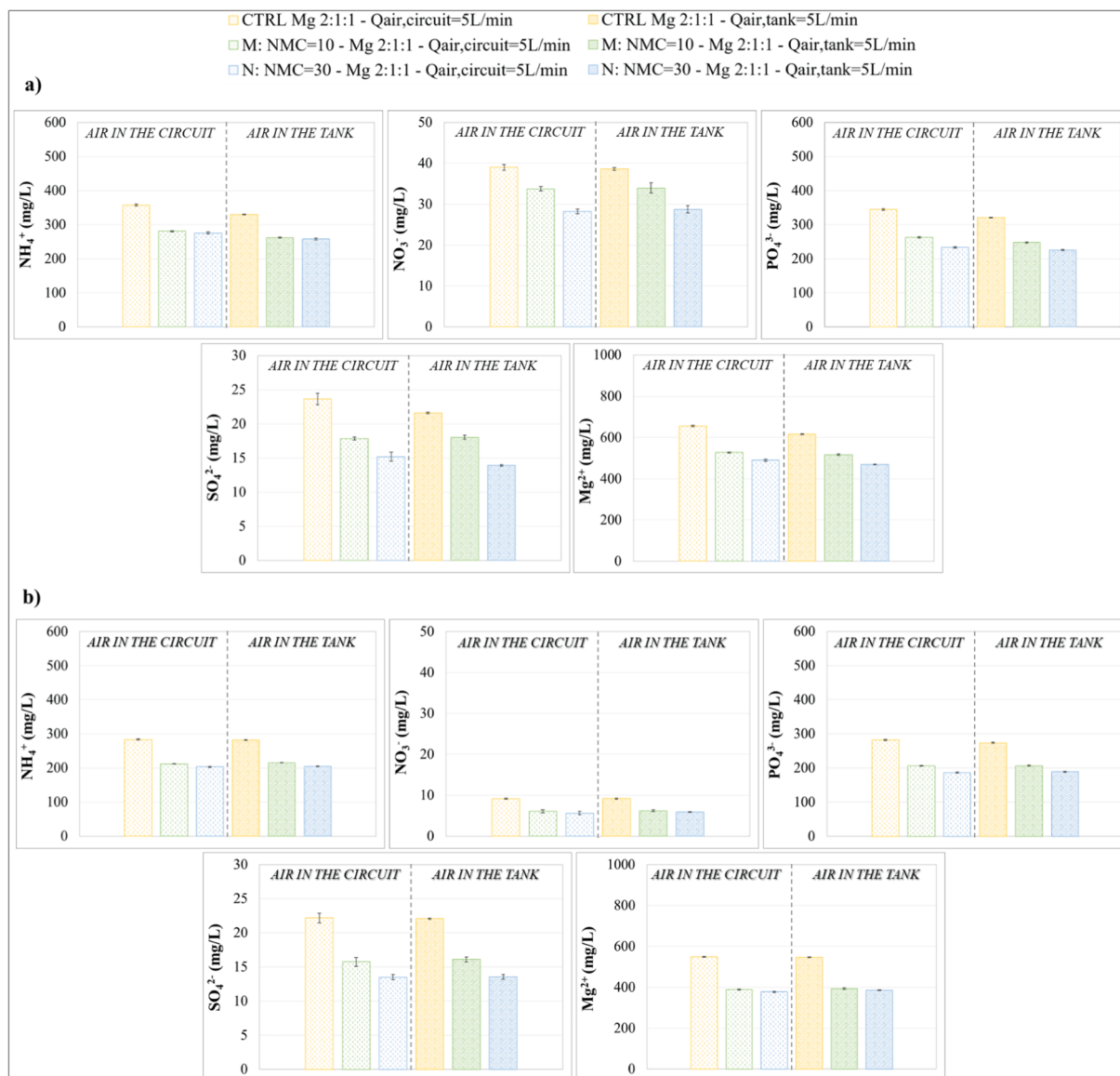
Fig. 6. \text{NH}_4^+ , \text{NO}_3^- , \text{PO}_4^{3-} , \text{SO}_4^{2-} , \text{Mg}^{2+} concentrations in HSAD digestate (a) and in AD digestate (b) obtained at the end of the magnetization treatment with the two different aeration strategies tested.
