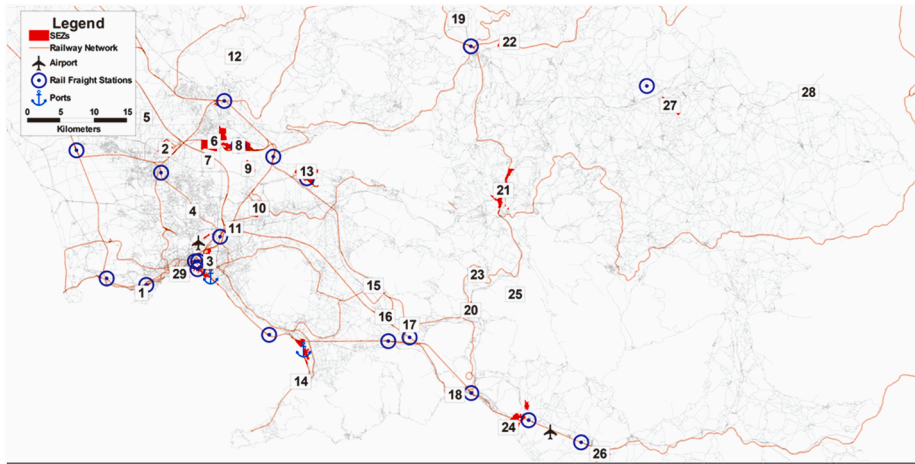
Fig. 4. SEZ areas and rail freight stations.
