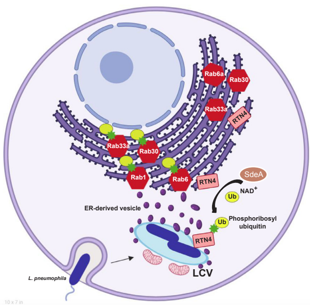
Fig. 3. Schematic representation of Legionella pneumophila infection mediated by SdeA effector. By transferring a phosphoribosyl group on ER-resident substrates, such Reticulon-4 (RTN4) and several Rab proteins, SdeA induces the formation of ER-derived vesicles and their association with the Legionella-containing vacuoles (LCVs). LCVs also make contacts with ER and mitochondria, a phenomenon that affects physiological processes, such as ER-phagy and mitophagy.
