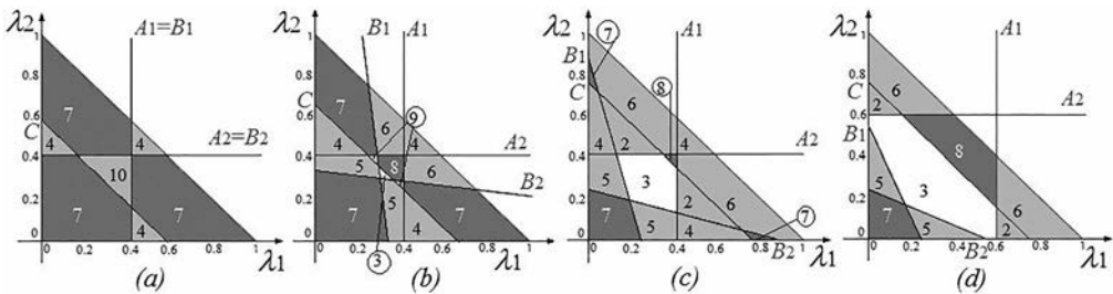
Figure 2. Examples of possible configurations of trade costs giving rise to different trade network configurations. Here a = b = c = 1/3 , E = 10 and T_U = T_{EX} = 0.325 in (a); T_U = 0.325 and T_{EX} = 0.37 in (b); T_U = 0.325 and T_{EX} = 0.45 in (c); and T_U = 0.25 and T_{EX} = 0.45 in (d).
