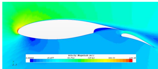
Figure 14: Fowler flap design: flap 20 deg. CFD velocity magnitude contour, M=0.17 Re=13.7e6 \alpha = 15^\circ
