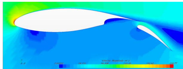
Figure 16: Fowler flap design: flap 35 deg. CFD velocity magnitude contour, M=0.154 Re=16.0e6 \alpha = 15^\circ
