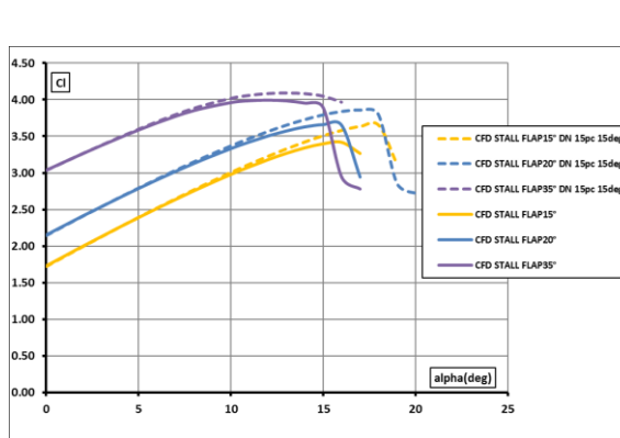
Figure 18: Kink flap section, effect of droop nose on lift coefficient, CFD results
