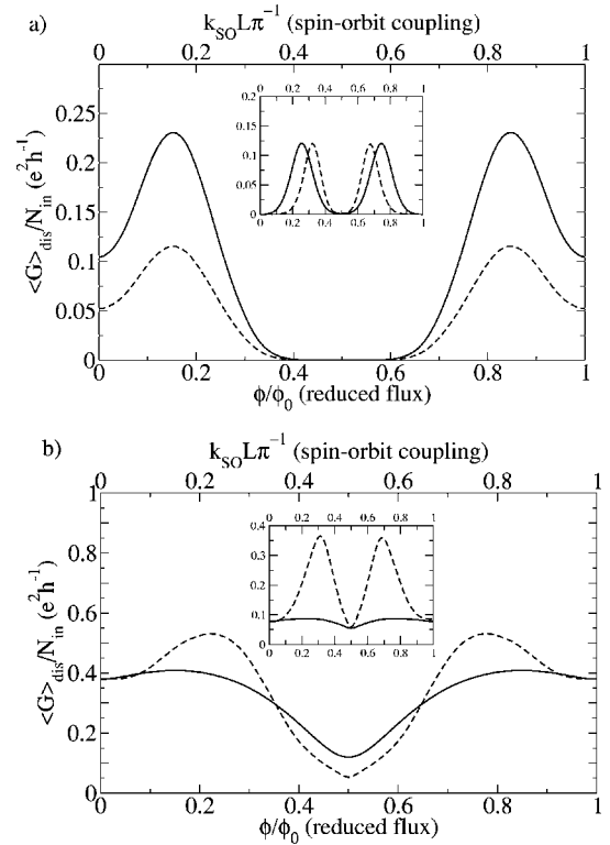
FIG. 3. Panel (a): Disorder-averaged conductance per channel, \langle G \rangle_{\text{dis}}/N_{\text{in}} , as a function of the reduced flux for zero spin-orbit coupling (solid line), and of spin-orbit coupling for zero magnetic field (dashed line), for the diamond chain with ten elementary squares. Panel (b): Disorder-averaged conductance per channel, \langle G \rangle_{\text{dis}}/N_{\text{in}} , as a function of the reduced flux for zero spin-orbit coupling (solid curve), and of spin-orbit coupling for zero magnetic field (dashed curve), for the ladder with ten elementary squares. In both panels, the injection wave vector is uniformly distributed in [k_F - \pi/2L, k_F + \pi/2L] with k_FL = 100 , and the disorder strength is \Delta L/L = 0.01 for the main panel, and \Delta L/L = 0.05 for the inset.
