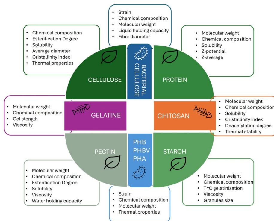
Figure 4. Physico-chemical properties of plant-, animal-, and microbial-origin biopolymers.
